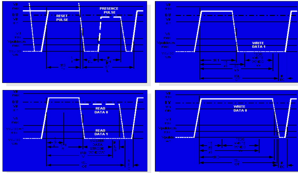
IEEE 1451.4 MMI Data Transmission Waveforms
